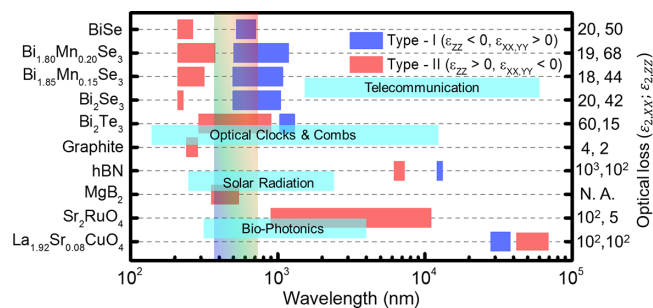
FIG. 4. Hyperbolic wavelength bands in natural materials. Blue and orange colors correspond to the bands with type-I and type-II hyperbolic medium, respectively. The top four lines ( \text{BiSe} , \text{Bi}_2\text{Se}_3 , and Mn doped \text{Bi}_2\text{Se}_3 ) represent that the hyperbolic materials are compared with other well-known natural hyperbolic material. The vertical "spectrum bar" indicates the wavelength range corresponding to visible light. The horizontal bar indicates the wavelength range for the application. The y-scale at the right side indicates the maximum optical loss along in-plane and the cross-plane ( \epsilon_{2,xx} and \epsilon_{2,zz} ) directions, respectively.
