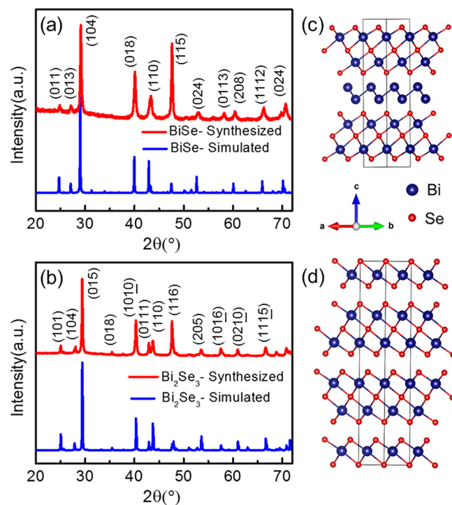
FIG. 1. Powder x-ray diffractogram of as-synthesized (red line) and simulated (blue line) (a) \text{BiSe} and (b) \text{Bi}_2\text{Se}_3 crystals is presented. The crystal structure of (c) \text{BiSe} and (d) \text{Bi}_2\text{Se}_3 is shown. Blue and red atoms represent Bi and Se atoms, respectively, in the \text{BiSe} and \text{Bi}_2\text{Se}_3 layers.
